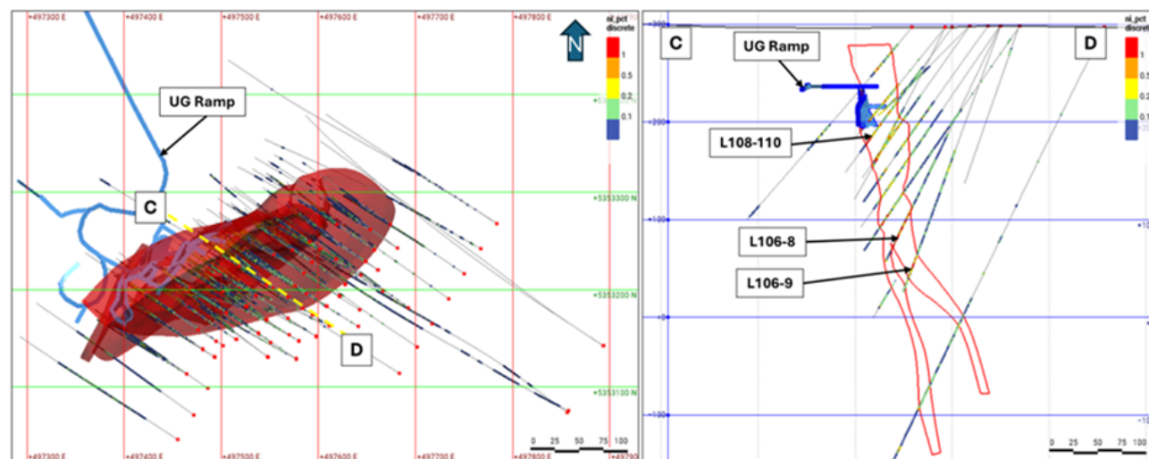
Figure 10.2 Aurora South Deposit Drillholes Layout in Plan and Typical Section
