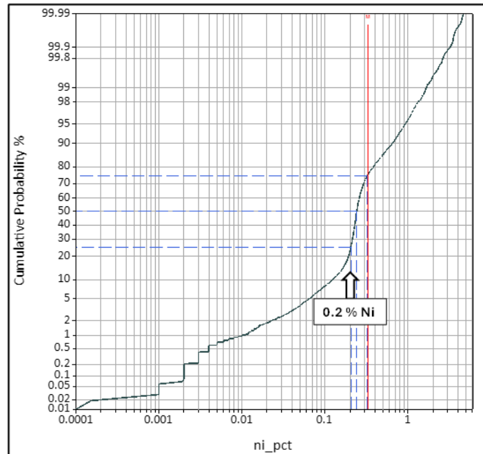
Figure 14.1 Log-probability Plot for Raw Ni values for the Aurora North Deposit
