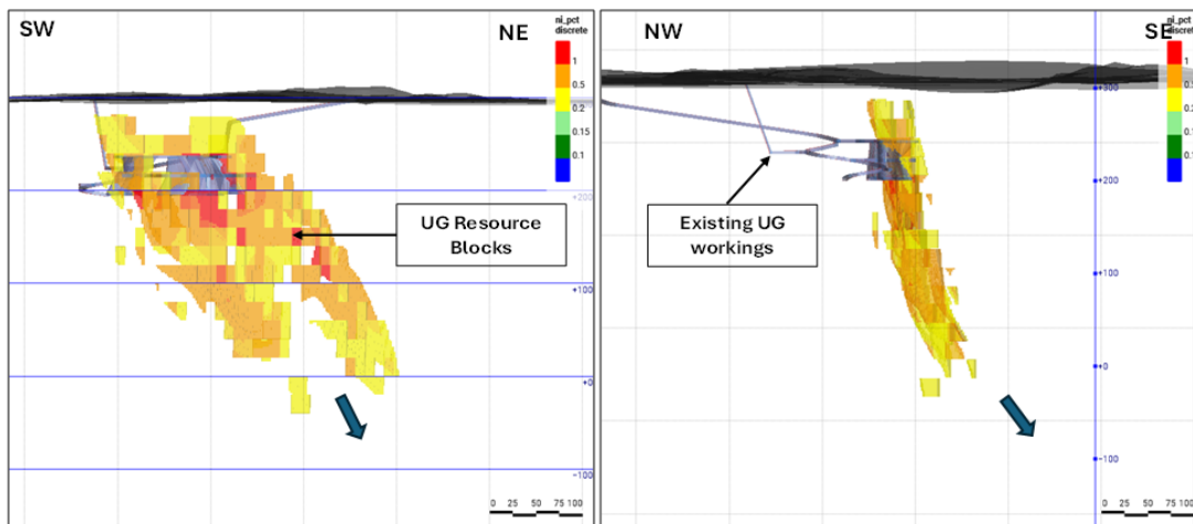
Figure 14.20 Aurora South Deposit UG Resource Blocks
