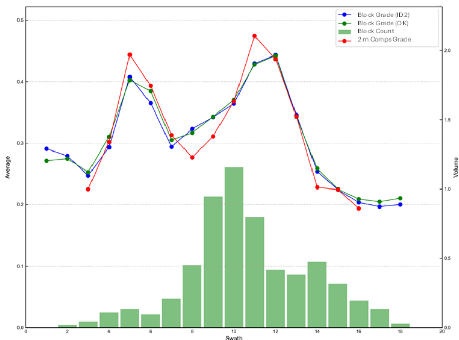
Figure 14.7 Swath Plot Along Easting (2 Block Spacing) for Ni Within the Main Zone
