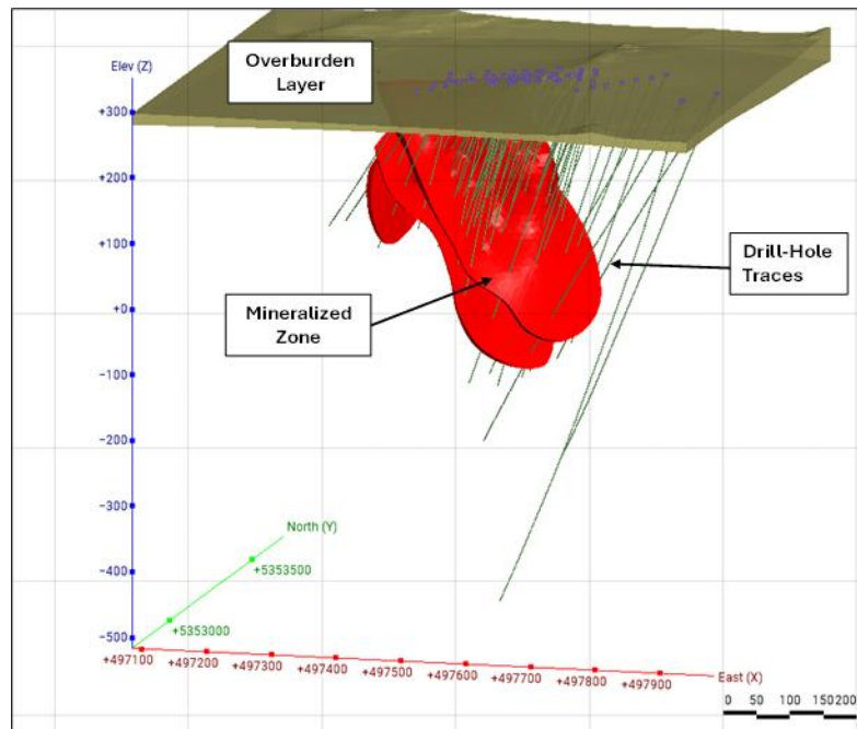
Figure 14.10 Isometric View of the Aurora South Deposit Mineralized Domain/Envelope
