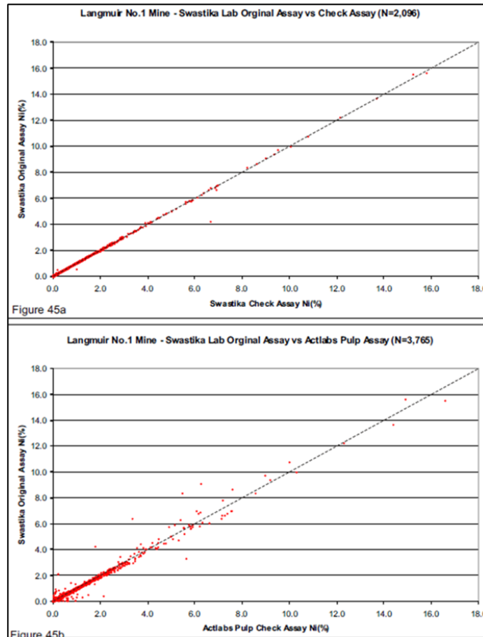
Figure 11.4 Duplicate and Repeat Analysis Results for Ni for Aurora South Deposit
