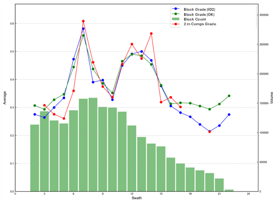
Figure 14.16 Swath Plot Along Depth (1 Block Spacing) for Ni Within Main Zone
