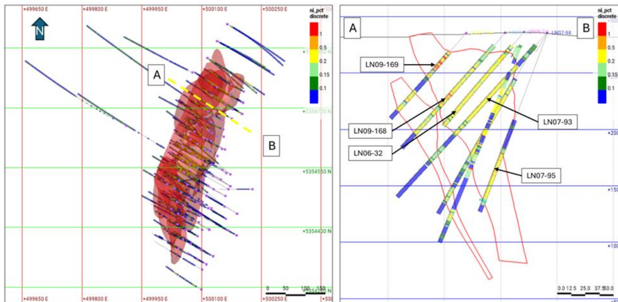
Figure 10.2 Aurora South Deposit Drillholes Layout in Plan and Typical Section
