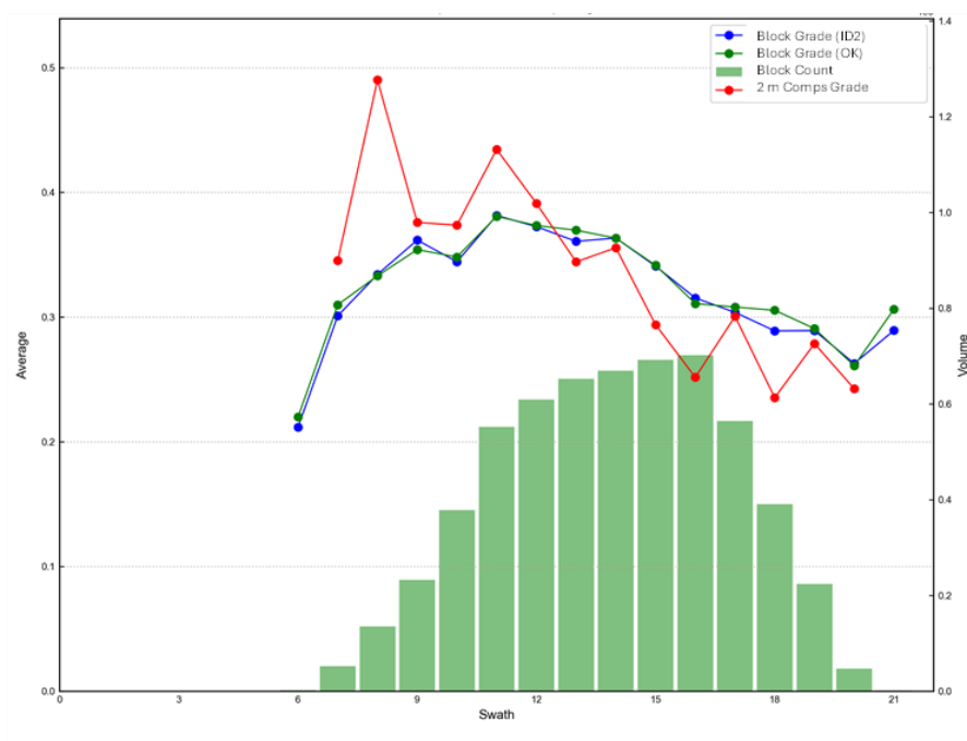
Figure 14.6 Swath Plot Along Northing (1 Block Spacing) for Ni Within Main Zone
