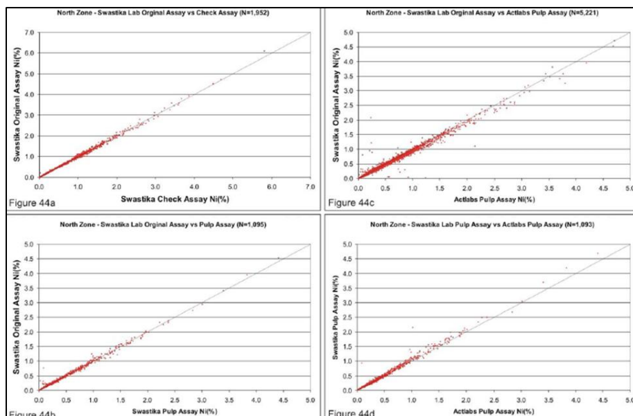
Figure 11.3 Duplicate and Repeat Analysis Results for Ni for Aurora North Deposit
