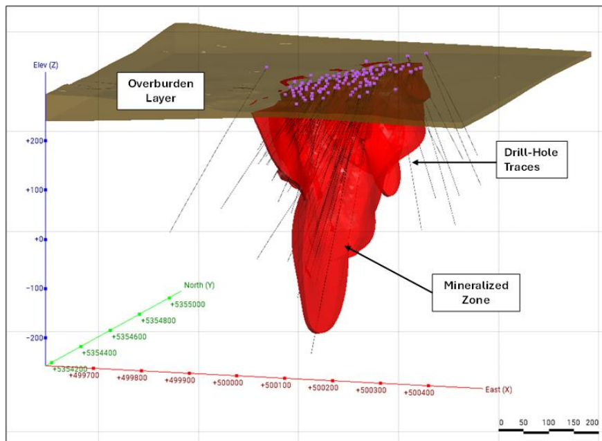
Figure 14.2 Isometric View of the Modelled Aurora North Deposit
