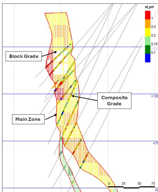
Figure 14.13 Typical Section Through the Aurora South Block Model Comparing Block Grades and Composite Grades
