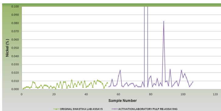
Figure 11.2 Blank Sample Control Chart for Aurora North and Aurora South
