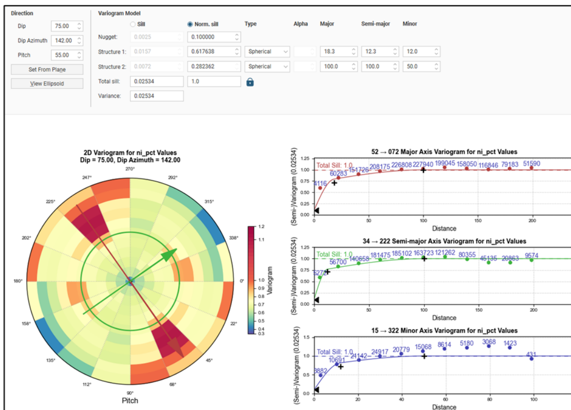
Figure 14.12 Aurora South Main Zone Variograms for Ni
