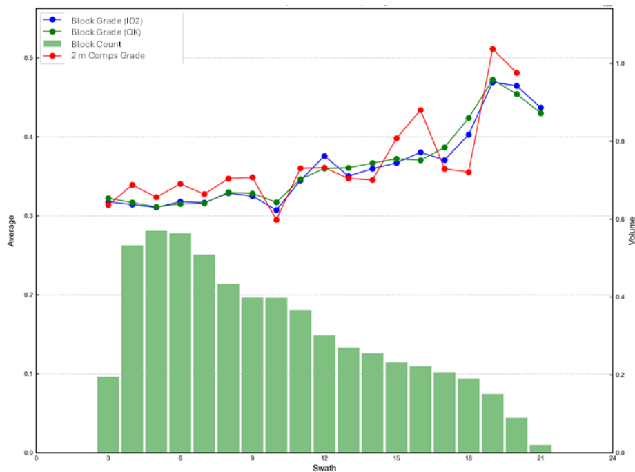
Figure 14.8 Swath Plot Along Depth (1 Block Spacing) for Ni Within the Main Zone
