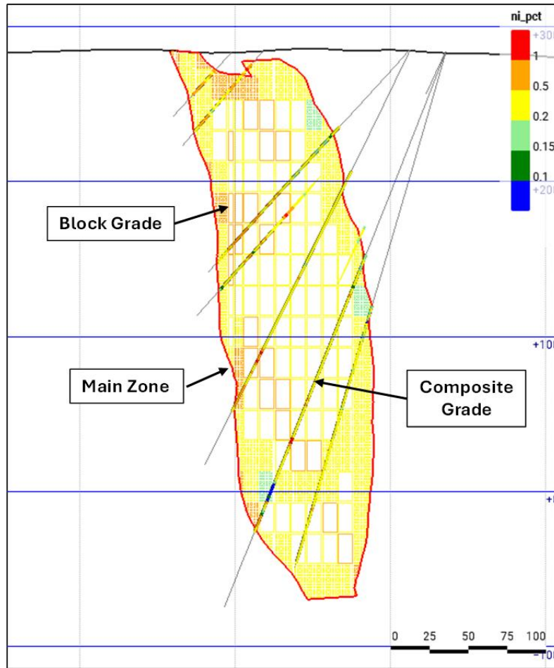
Figure 14.5 Typical Section Through the Aurora North Block Model Comparing Block Grades and Composites Grades
