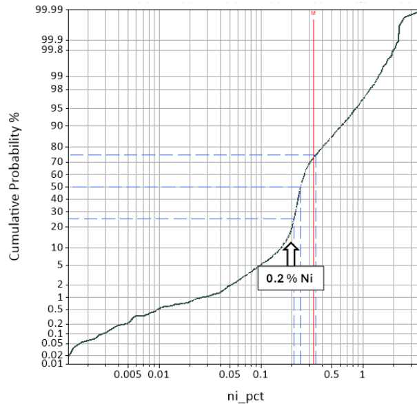
Figure 14.9 Log-probability Plot for Raw Ni Values for the Aurora South Deposit
