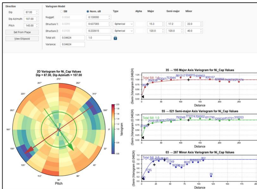
Figure 14.4 Aurora North Main Zone Variograms for Ni
