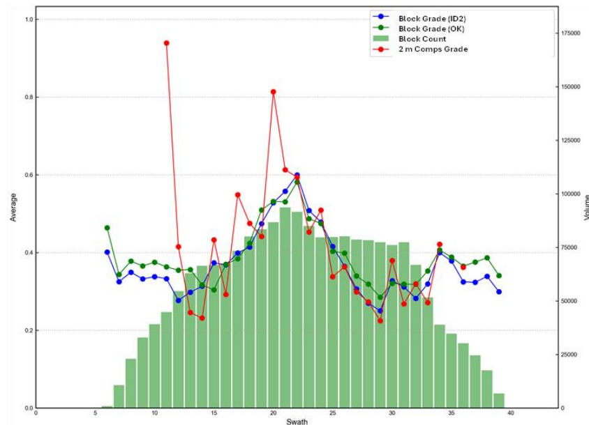
Figure 14.14 Swath Plot Along Northing (1 Block Spacing) for Ni Within the Main Zone
