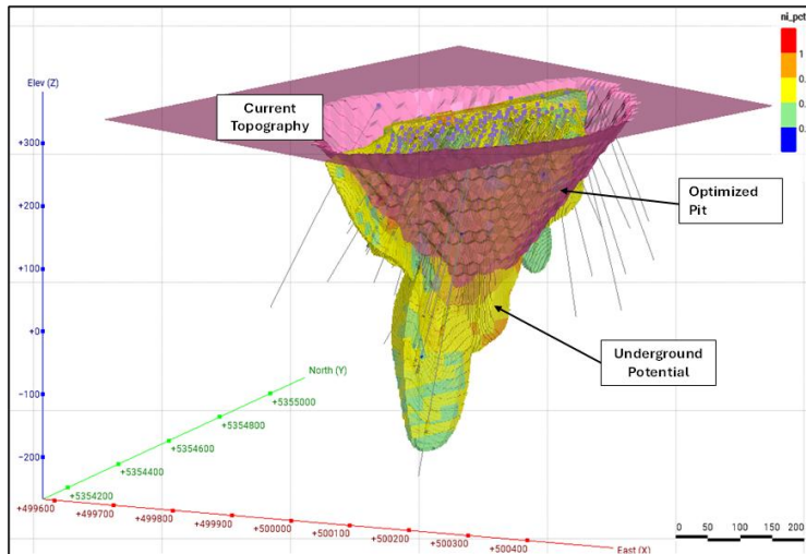
Figure 14.20 Aurora South Deposit UG Resource Blocks
