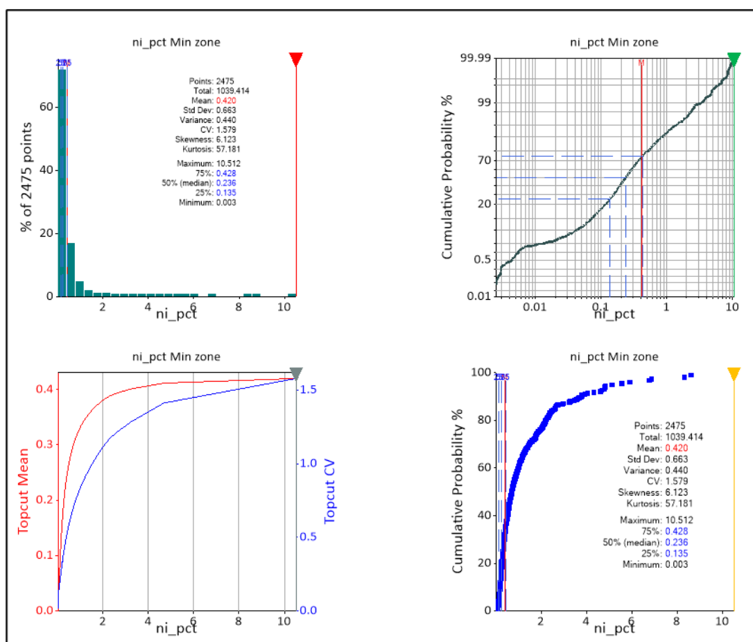
Figure 14.11 Statistical Plots Showing of Ni Composite Values Within the Mineral Domain/Envelope
