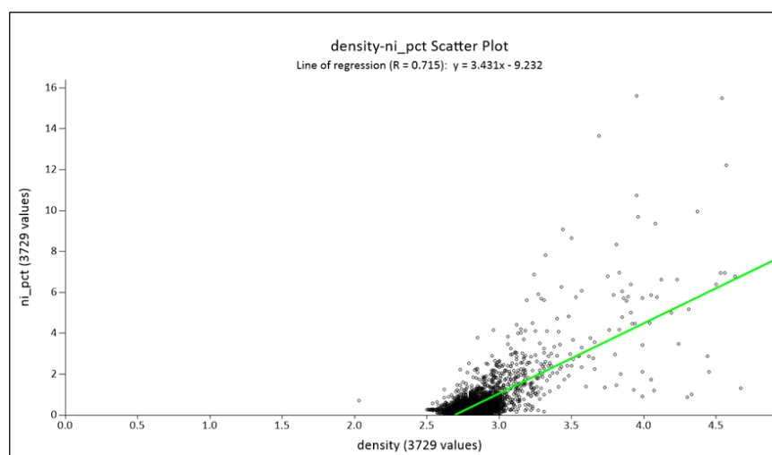
Figure 14.17 Comparison of Bulk Density versus Ni Grade for Aurora South Deposit
