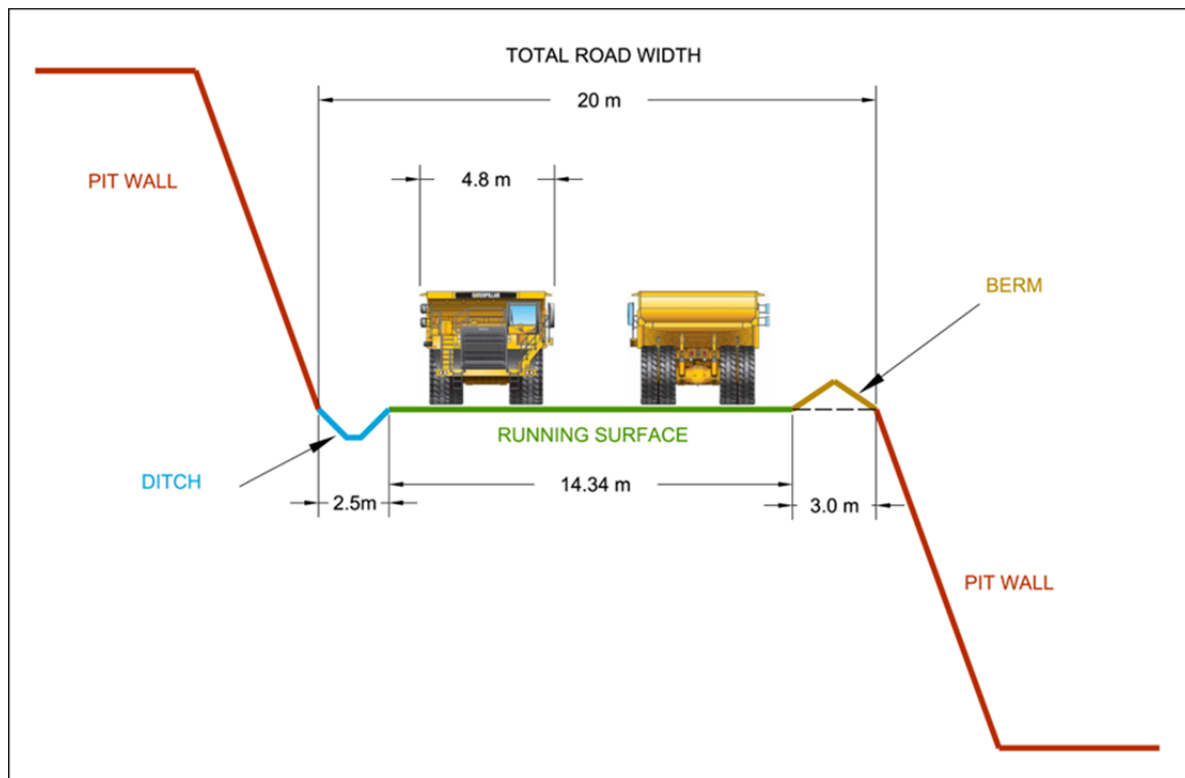
Figure 16-8: Ramp Design
