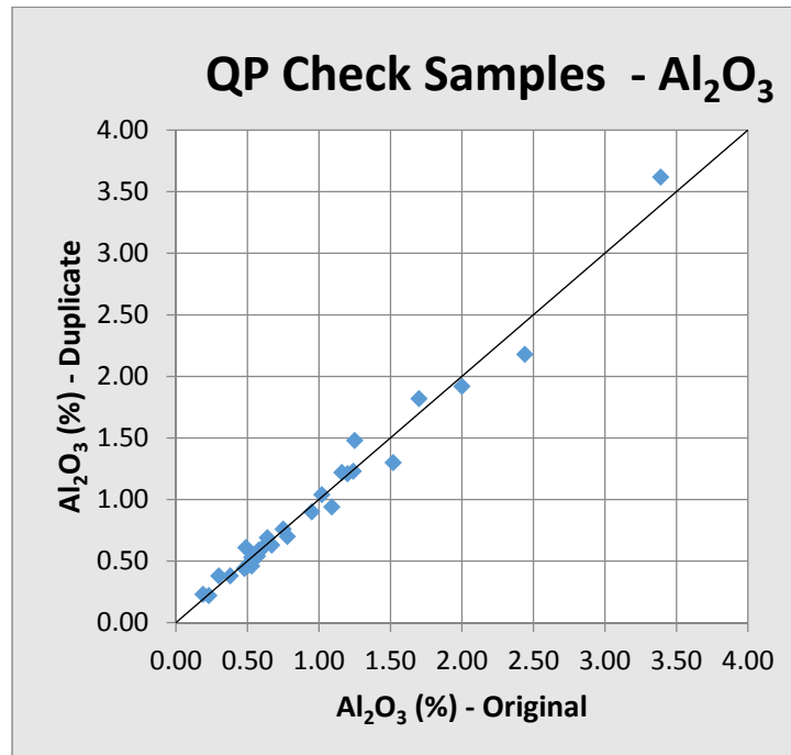
Figure 12-1: Independent Check Samples – \text{Al}_2\text{O}_3 Analyses of Original and Duplicate Samples
