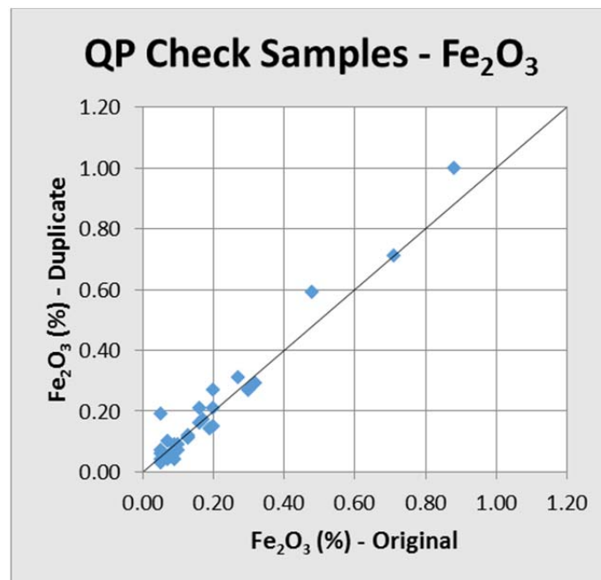
Figure 12-2: Independent Check Samples, \text{Fe}_2\text{O}_3 Analyses of Original and Duplicate Samples
