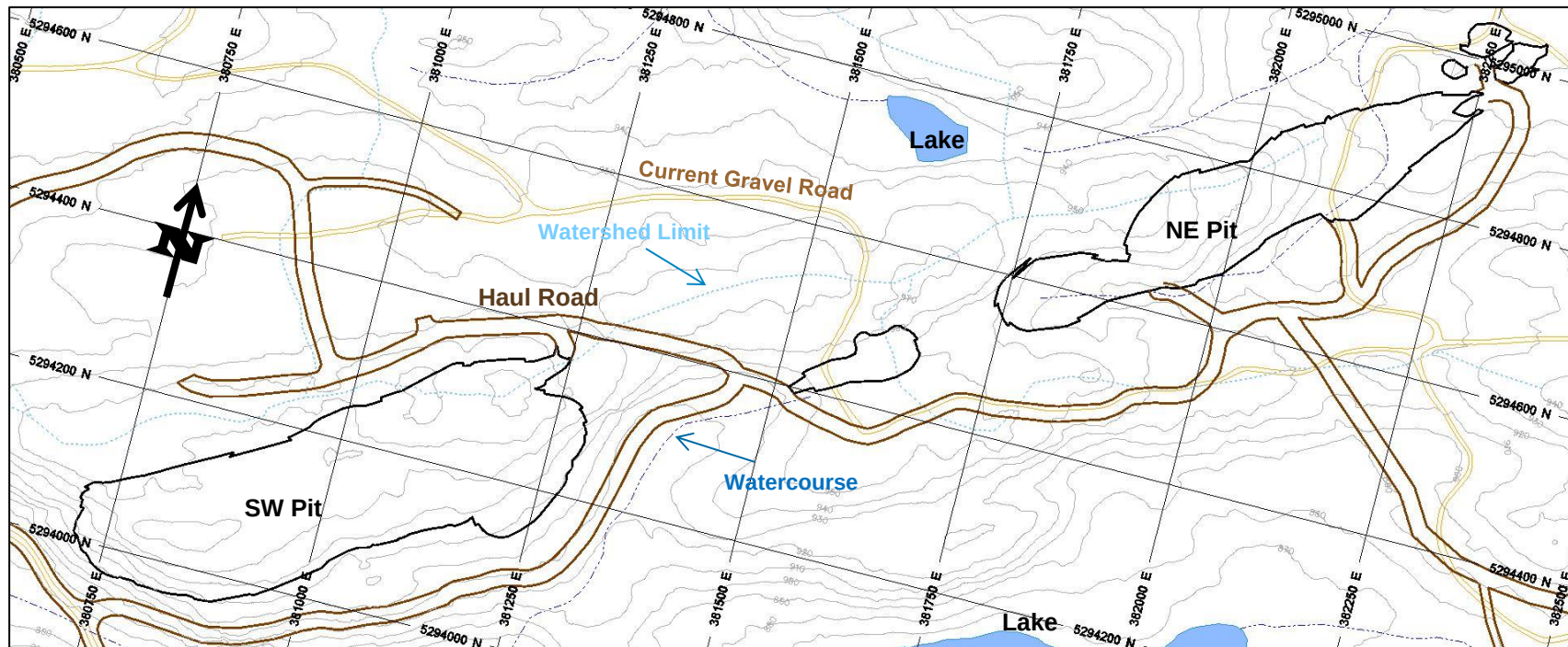
Mine Layout with SW & NE Pit Limits (10 m Contours)
