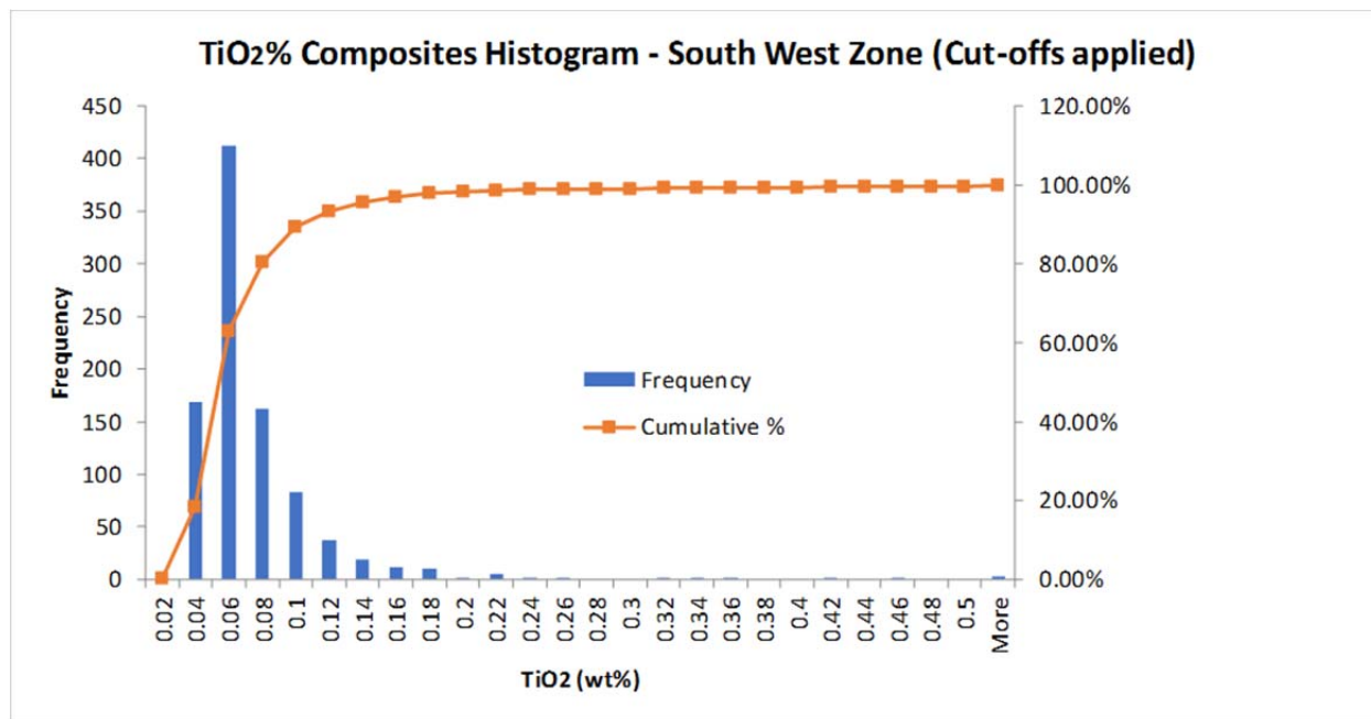
Figure 14-6 Composites histogram on \text{TiO}_2\% for the South West Zone
