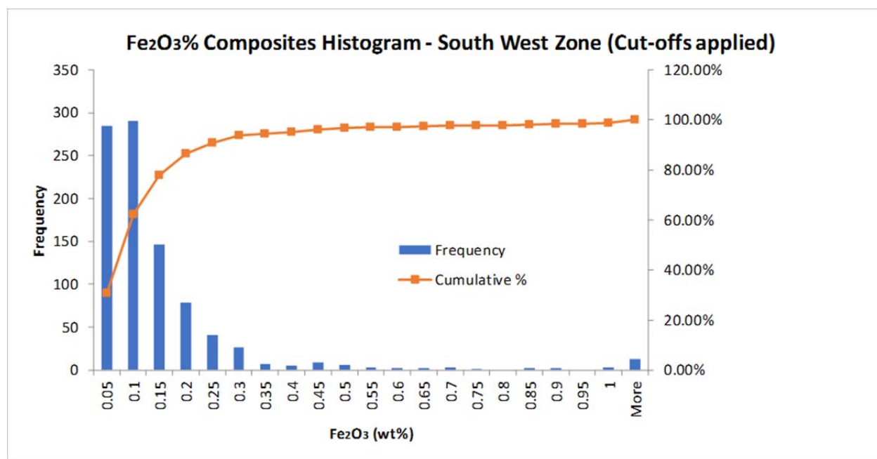
Figure 14-7 Composites histogram on \text{Fe}_2\text{O}_3\% for the South West Zone
