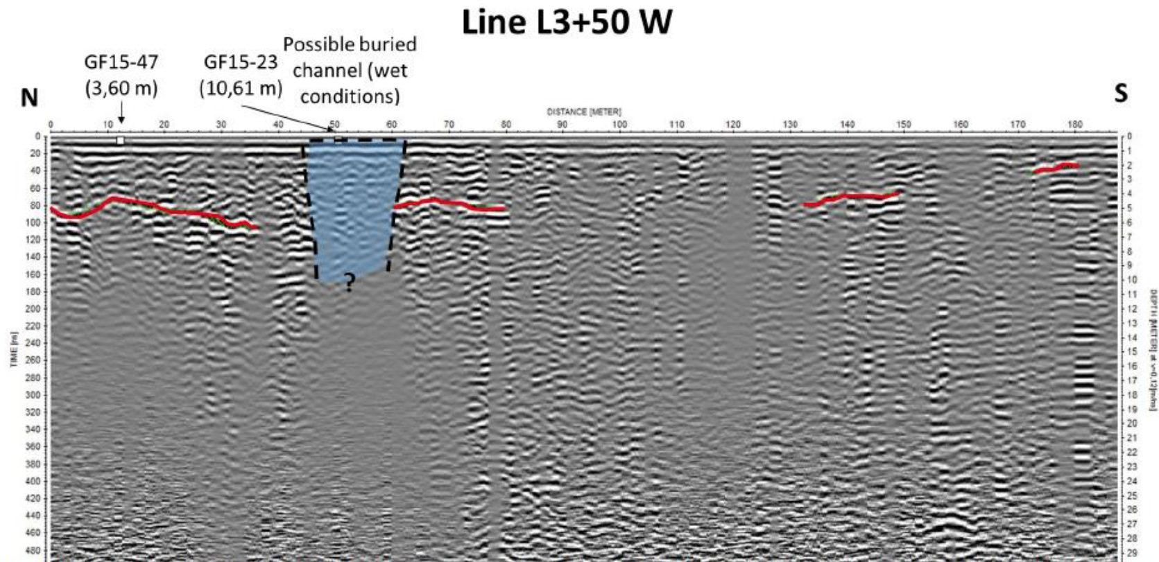
Figure A 5 : GPR profile along line L3+50 W with reflectors interpreted as bedrock (red lines) and drill hole location with overburden thickness estimates. Note the presence of wet conditions and a feature interpreted as a possible buried channel in bedrock.
