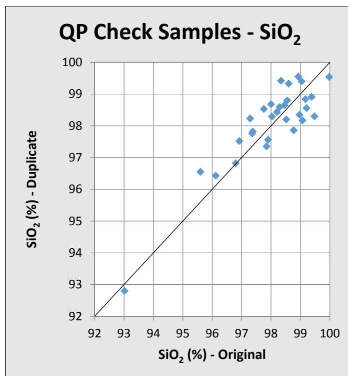
Figure 12-4: Independent Check Samples, \text{SiO}_2 Analyses of Original and Duplicate Samples
