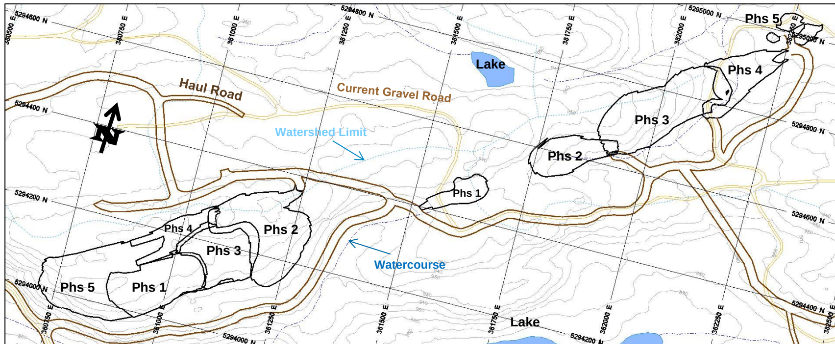
Mine Layout with SW & NE Phased Pit Limits (10 m Contours)
