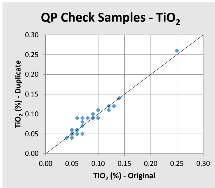
Figure 12-3: Independent Check Samples, \text{TiO}_2 Analyses of Original and Duplicate Samples
